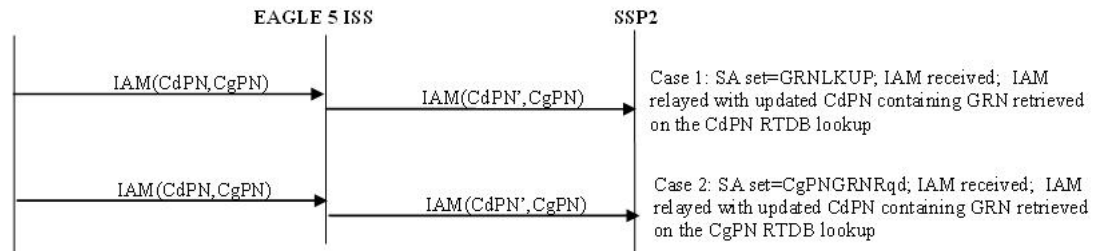
Figure 2-22 ISUP IAM Message Flows for TIF GRN for TIF CdPN Service
