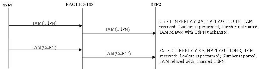
Figure 2-1 ISUP Message Flows for TIF NP CdPN Relay
